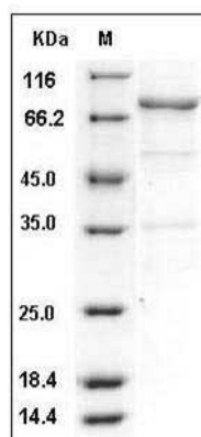
Human c-Yes / YES1 Protein (His & GST Tag) SDS-PAGE
