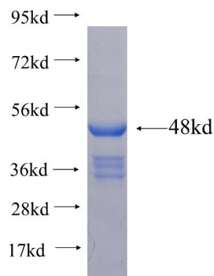
Recombinant Arabidopsis thaliana NIM1 SDS-PAGE
