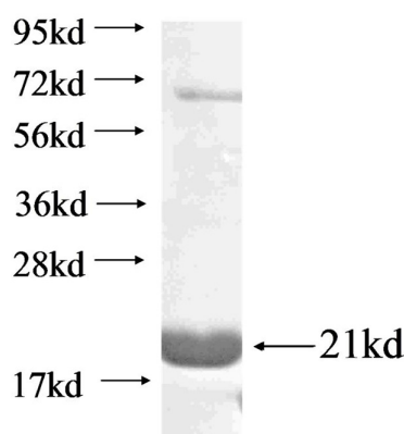
Recombinant Arabidopsis thaliana NRG1A SDS-PAGE
