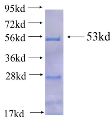
Recombinant Arabidopsis thaliana HCT SDS-PAGE
