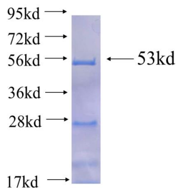
Recombinant Arabidopsis thaliana HCT SDS-PAGE
