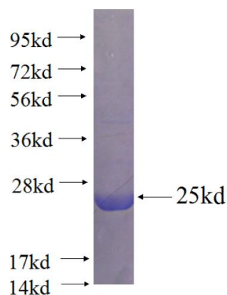
Recombinant Arabidopsis thaliana BAL SDS-PAGE
