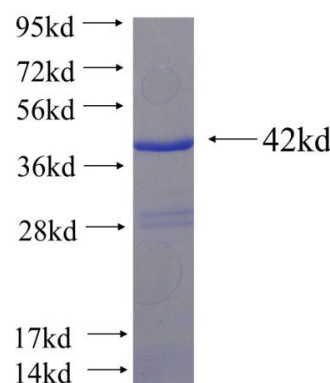
Recombinant Arabidopsis thaliana DCA1 SDS-PAGE
