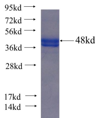
Recombinant Arabidopsis thaliana AtGAP1 SDS-PAGE
