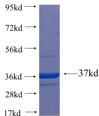
Recombinant Arabidopsis thaliana ATFD2 SDS-PAGE
