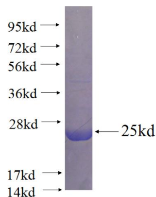
Recombinant Arabidopsis thaliana AVDE1 SDS-PAGE
