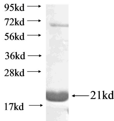
Recombinant Arabidopsis thaliana IRP7 SDS-PAGE
