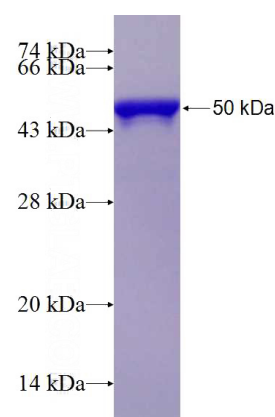
Recombinant Human MYH9 SDS-PAGE
