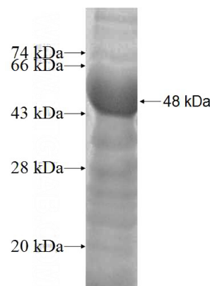
Recombinant Human SSFA2 SDS-PAGE
