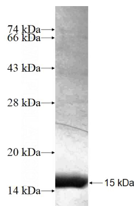
Recombinant Human KCNT2 SDS-PAGE
