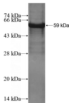
Recombinant Human FAM135B SDS-PAGE
