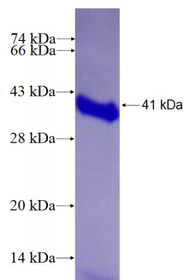
Recombinant Human NRIP1 SDS-PAGE
