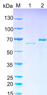
Recombinant Human STK31 SDS-PAGE
