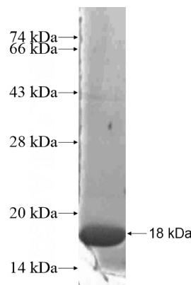
Recombinant Human HEATR2 SDS-PAGE
