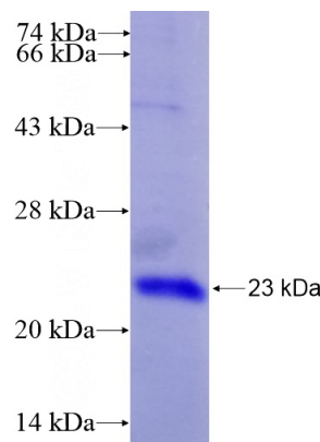
Recombinant Human TLR1 SDS-PAGE
