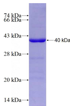
Recombinant Human NFkB2 SDS-PAGE
