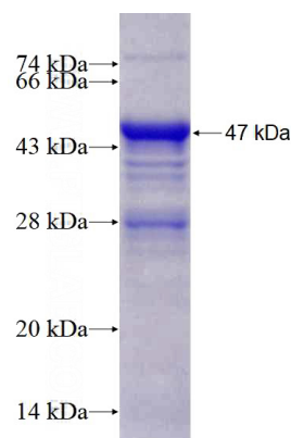
Recombinant Human UBN1 SDS-PAGE
