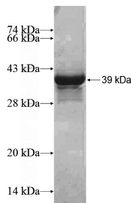
Recombinant Human EXOSC10 SDS-PAGE
