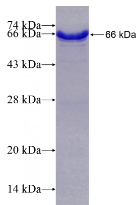
Recombinant Human WDR24 SDS-PAGE
