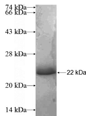
Recombinant Human SLC38A10 SDS-PAGE
