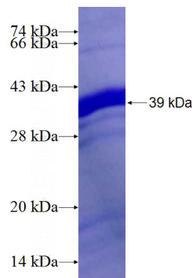
Recombinant Human KAT2A SDS-PAGE
