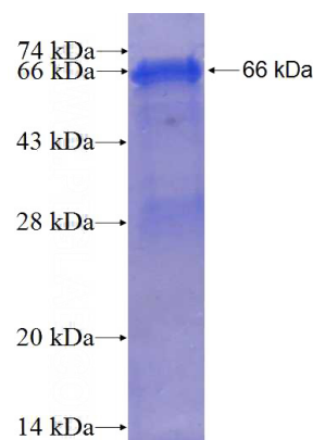
Recombinant Human MTHFD1 SDS-PAGE
