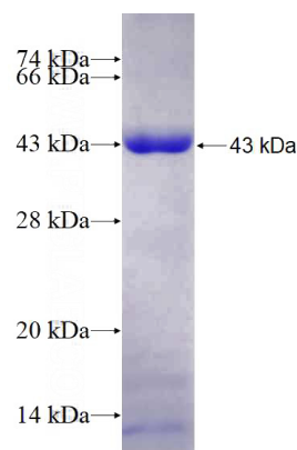
Recombinant Human MCM4 SDS-PAGE
