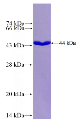
Recombinant Human RNF139 SDS-PAGE
