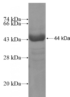
Recombinant Human SHROOM1 SDS-PAGE
