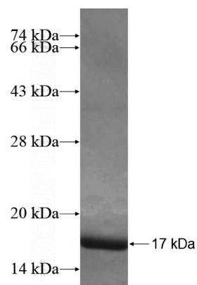
Recombinant Human SLC26A11 SDS-PAGE
