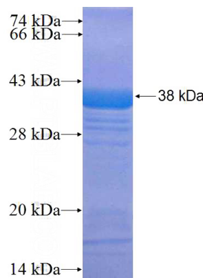
Recombinant Human PAK7 SDS-PAGE
