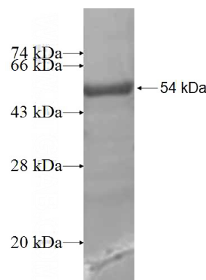
Recombinant Human SATB1 SDS-PAGE
