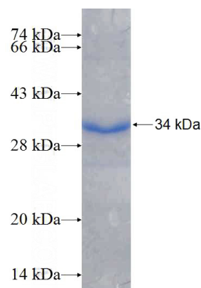
Recombinant Human ACSBG1 SDS-PAGE
