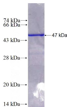
Recombinant Human PIK3CD SDS-PAGE
