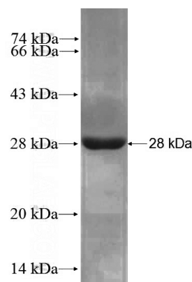
Recombinant Human ATP1A3 SDS-PAGE
