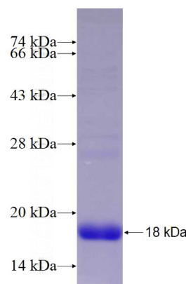
Recombinant Human GPR61 SDS-PAGE
