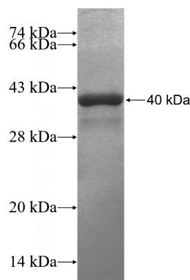
Recombinant Human AZIN1 SDS-PAGE
