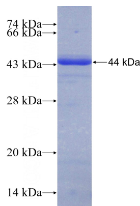
Recombinant Human C19orf21 SDS-PAGE
