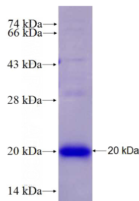
Recombinant Human KPNA3 SDS-PAGE
