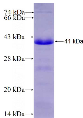
Recombinant Human CDH7 SDS-PAGE
