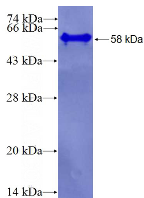
Recombinant Human WDR42A SDS-PAGE
