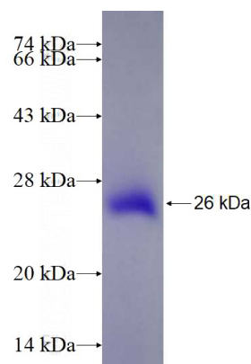
Recombinant Human RNF219 SDS-PAGE
