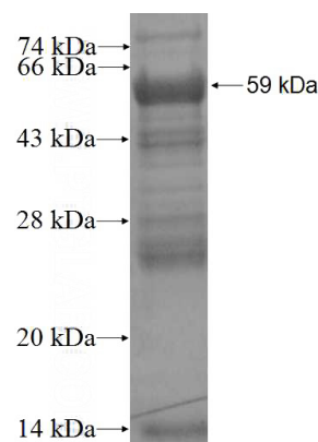
Recombinant Human ACRBP SDS-PAGE
