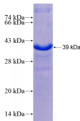
Recombinant Human ECM1 SDS-PAGE
