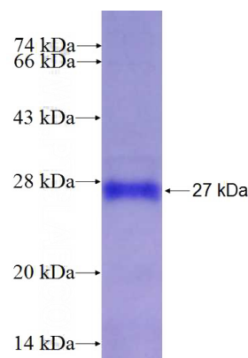
Recombinant Human SYDE1 SDS-PAGE
