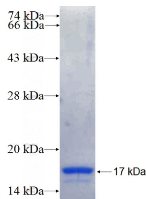
Recombinant Human USP4 SDS-PAGE
