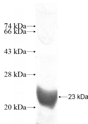
Recombinant Human SLC6A18 SDS-PAGE
