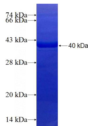
Recombinant Human EEPD1 SDS-PAGE
