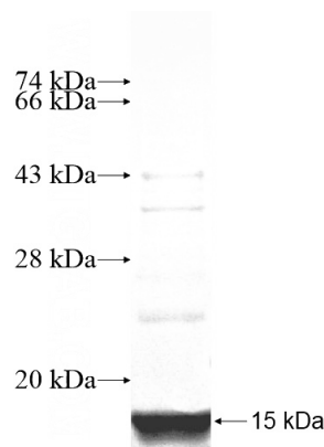
Recombinant Human SLC2A11 SDS-PAGE
