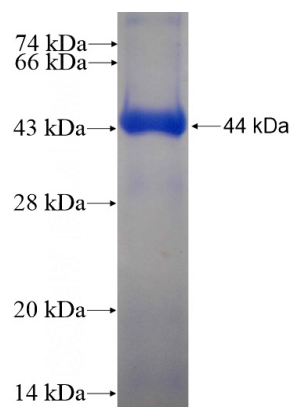
Recombinant Human ACOT12 SDS-PAGE
