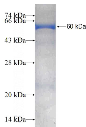
Recombinant Human FH SDS-PAGE
